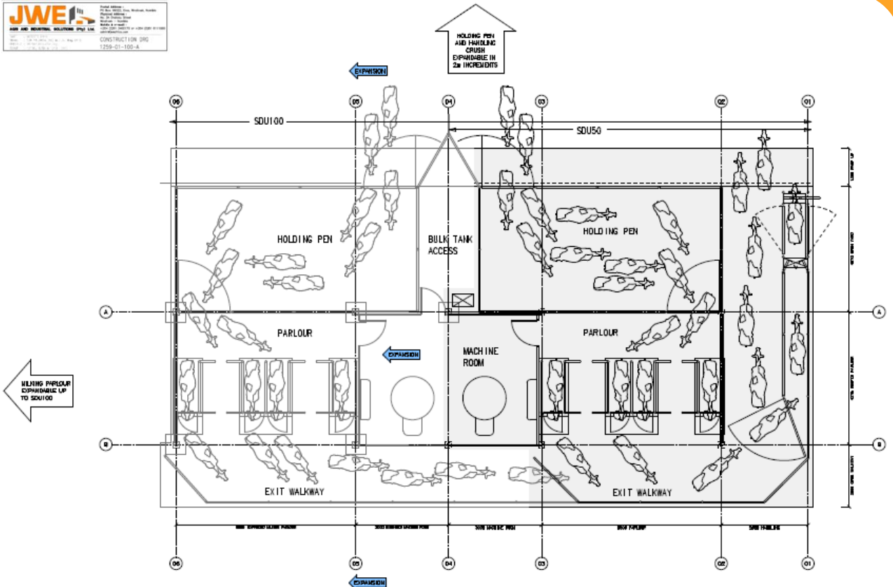
FLOOR PLAN - SDU/100
