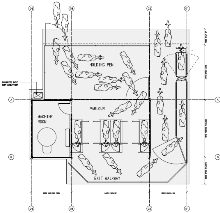
FLOOR PLAN - SDU/50
